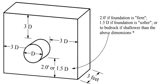
Figure 2 - Typical configuration of filter diaphragm used in the design of an embankment dam.
