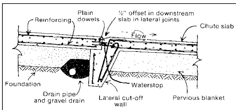
Figure 6 Typical Floor Lining on Earth (Soil) Foundations
