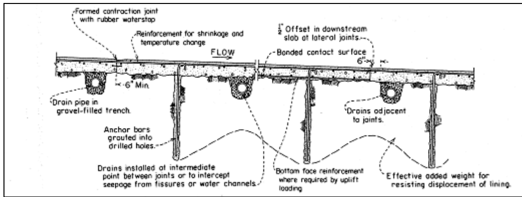
Figure 7 Typical Floor Lining on Rock Foundations
