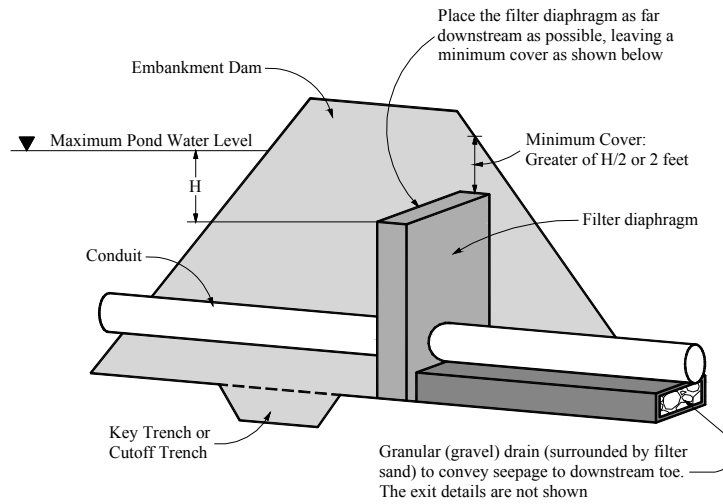
Figure 1 - Typical configuration for a filter diaphragm used in the design of an embankment dam. The figure shows the location of the filter diaphragm as far downstream as possible (downstream of key trench or cutoff trench), leaving adequate cover over it.
