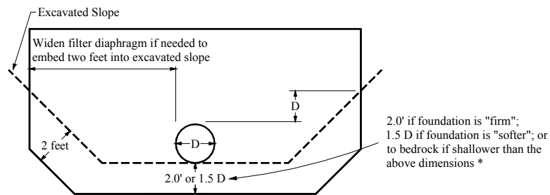
Figure 3 - Typical configuration for a filter diaphragm used in the design of an embankment dam. The filter diaphragm should extend into the foundation soils, where an excavation is made for the conduit.
